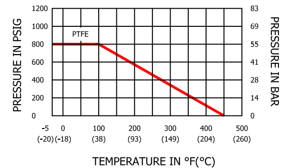
Pressure VS. Temperature Chart
